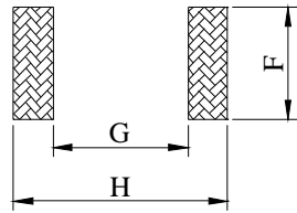
( PCB Pattern )
